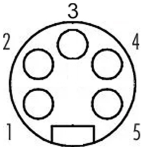
PIN LAYOUT, FACE VIEW (MATING SIDE), FEMALE
