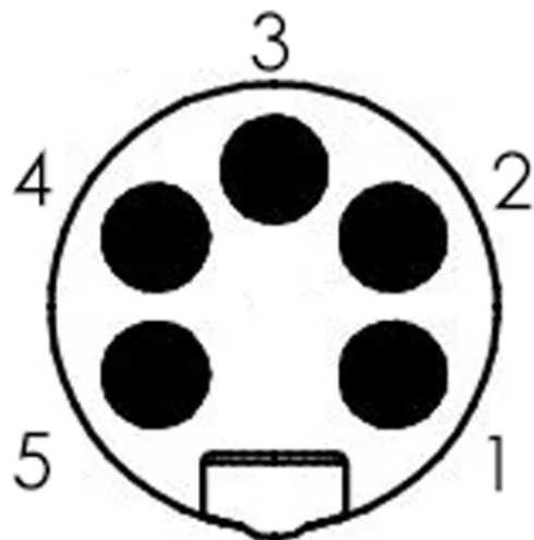
PIN LAYOUT, FACE VIEW (MATING SIDE), MALE
