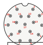
17-pin A-coded
