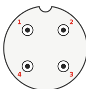
4-pin A-coded
