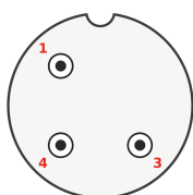
3-pin A-coded
