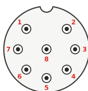
8-pin A-coded
