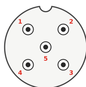
5-pin A-coded
