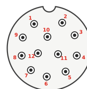
12-pin A-coded
