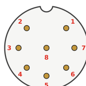
8-pin A-coded
