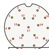
17-pin A-coded
