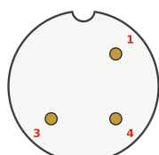
3-pin A-coded
