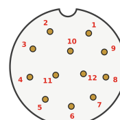
12-pin A-coded
