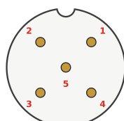
5-pin A-coded
