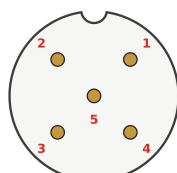
5-pin A-coded
