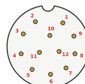
12-pin A-coded
