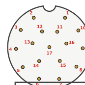
17-pin A-coded
