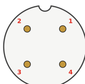
4-pin A-coded
