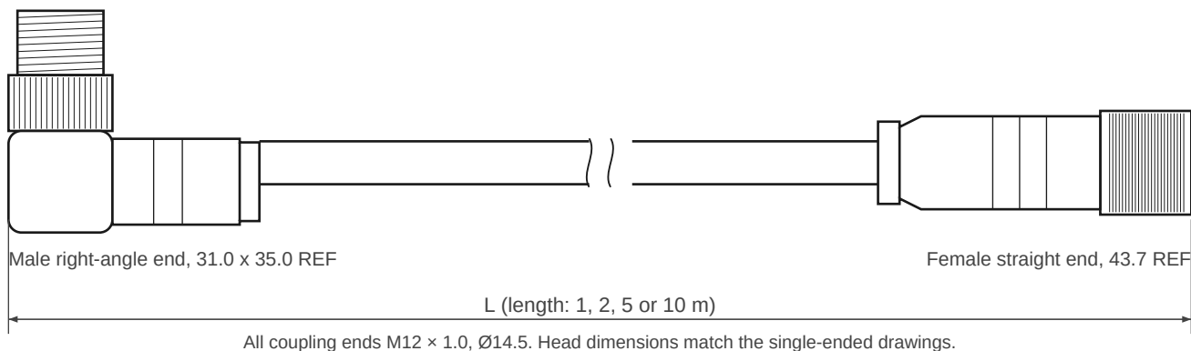
5-pin B-coded
