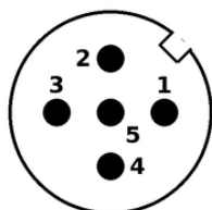
Male face view (mating side)
