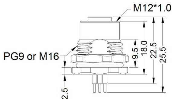
FEMALE, STRAIGHT, FRONT MOUNT
