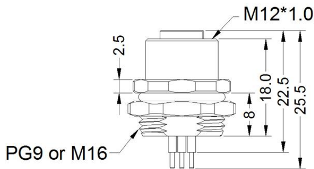
FEMALE, STRAIGHT, REAR MOUNT
