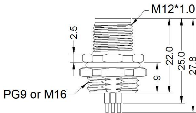
MALE, STRAIGHT, REAR MOUNT
