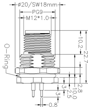
MALE, STRAIGHT, FRONT MOUNT
