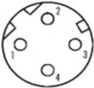
Female face view (mating side)
