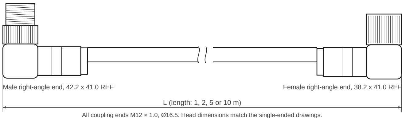
5-pin K-coded
