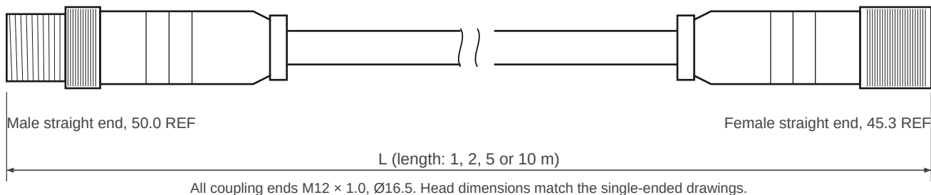
5-pin K-coded
