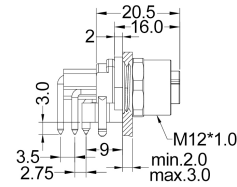
FEMALE, RIGHT-ANGLE, FRONT MOUNT
