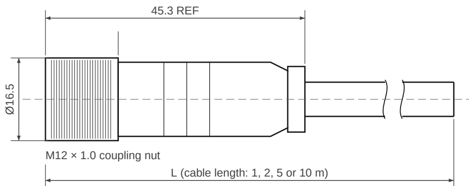
4-pin L-coded
