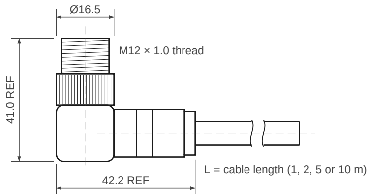
4-pin L-coded
