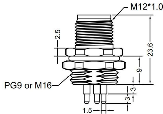
MALE, STRAIGHT, REAR MOUNT
