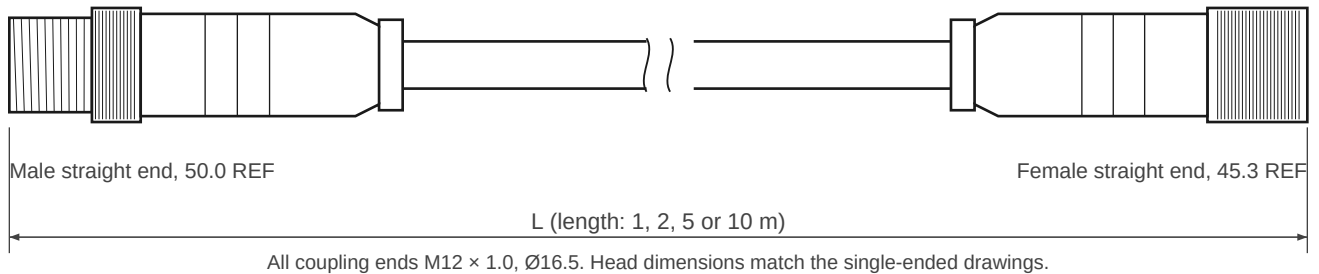
4-pin S-coded
