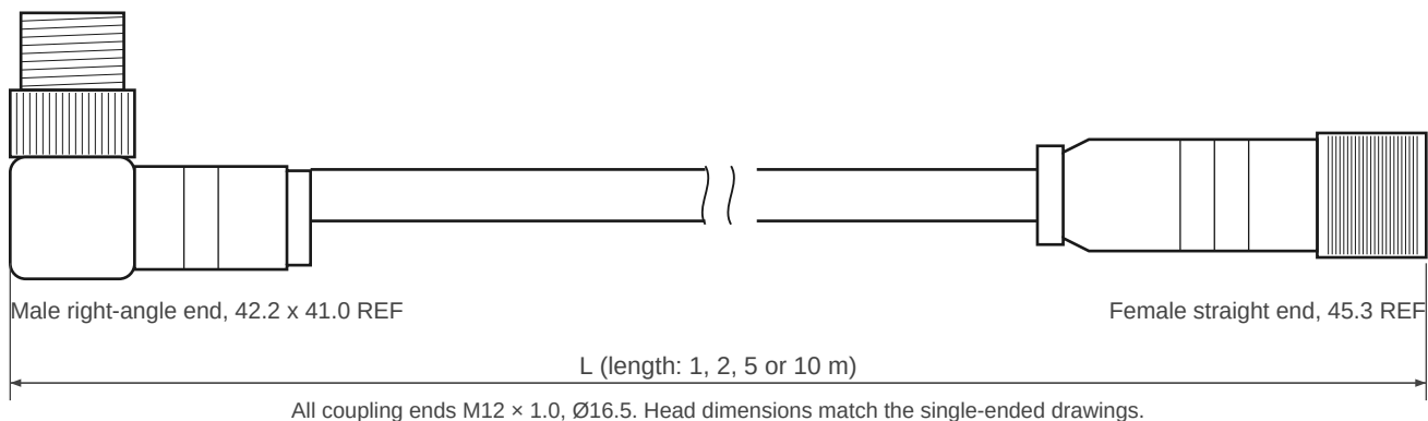
4-pin S-coded
