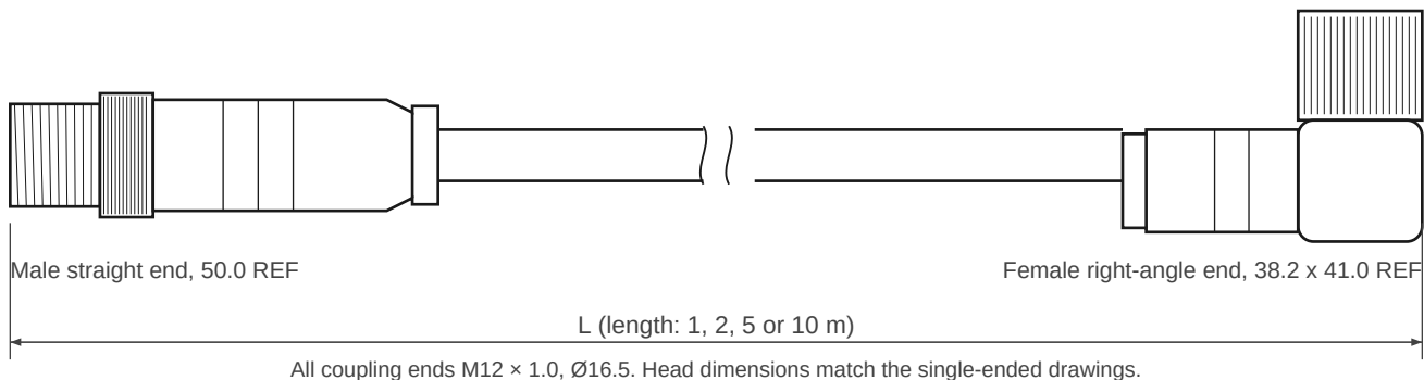
4-pin S-coded
