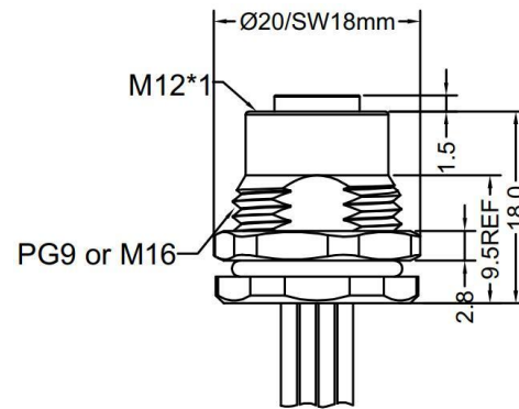
FEMALE, STRAIGHT, FRONT MOUNT
