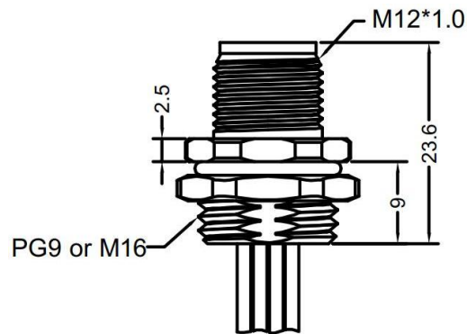
MALE, STRAIGHT, REAR MOUNT
