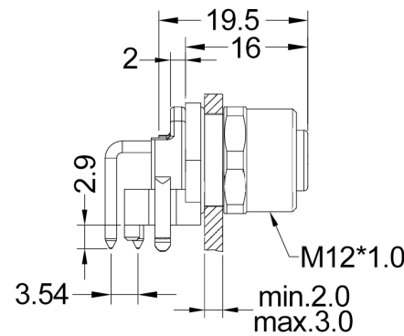
FEMALE, RIGHT-ANGLE, FRONT MOUNT
