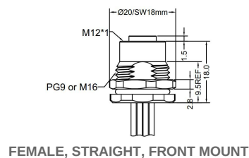
FEMALE, STRAIGHT, FRONT MOUNT
