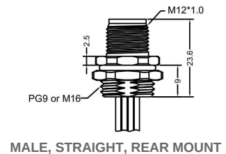
MALE, STRAIGHT, REAR MOUNT
