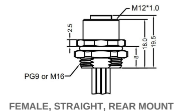
FEMALE, STRAIGHT, REAR MOUNT
