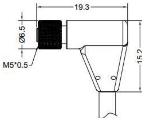
FEMALE RIGHT-ANGLE
