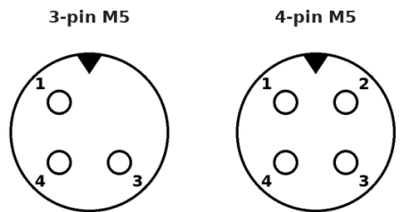
Female face view (mating side)
