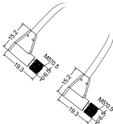
FEMALE RIGHT-ANGLE TO FEMALE RIGHT-ANGLE
