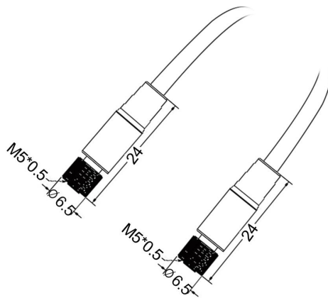
FEMALE STRAIGHT TO FEMALE STRAIGHT
