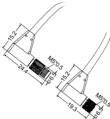
MALE RIGHT-ANGLE TO FEMALE RIGHT-ANGLE
