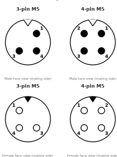
MALE RIGHT-ANGLE TO FEMALE RIGHT-ANGLE
