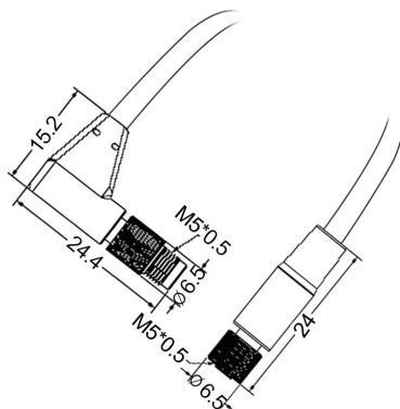
MALE RIGHT-ANGLE TO FEMALE STRAIGHT
