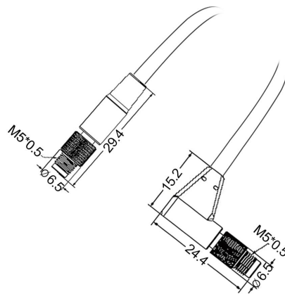
MALE STRAIGHT TO MALE RIGHT-ANGLE
