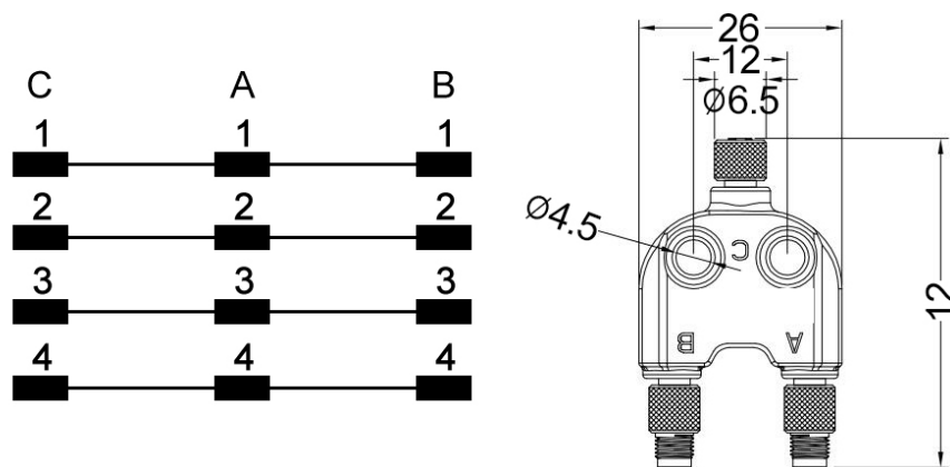
WIRING AND DIMENSIONS
