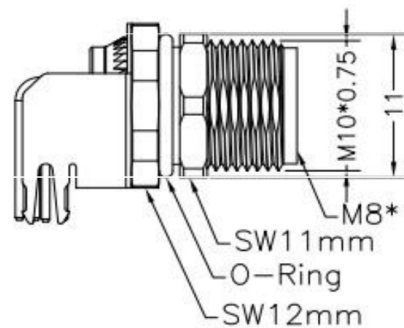
FEMALE, RIGHT-ANGLE, FRONT MOUNT
