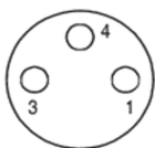
Female face view (mating side)
