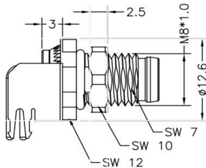
MALE, RIGHT-ANGLE, FRONT MOUNT
