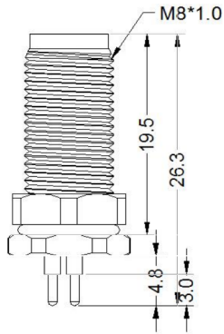
MALE, STRAIGHT, FRONT MOUNT
