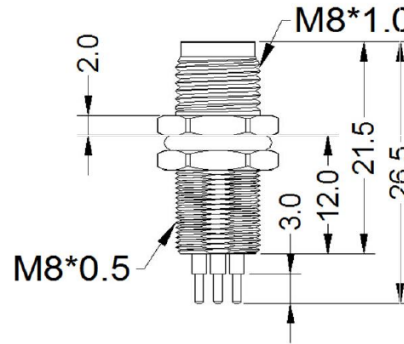
MALE, STRAIGHT, REAR MOUNT
