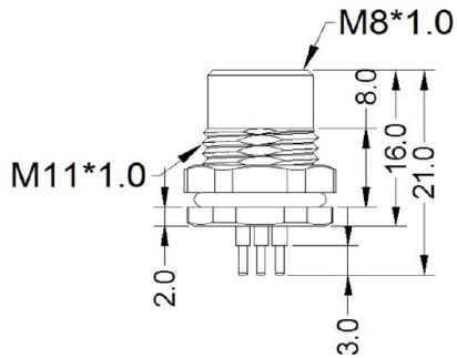
FEMALE, STRAIGHT, FRONT MOUNT
