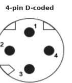
Male face view (mating side)
