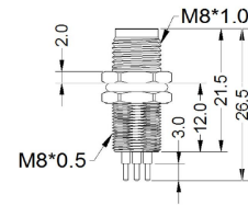
MALE, STRAIGHT, REAR MOUNT
