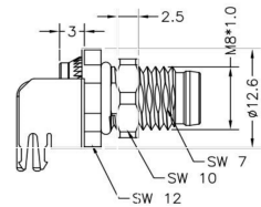
MALE, RIGHT-ANGLE, FRONT MOUNT
