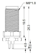
MALE, STRAIGHT, FRONT MOUNT
