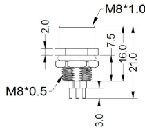
FEMALE, STRAIGHT, REAR MOUNT
