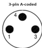
Male face view (mating side)
