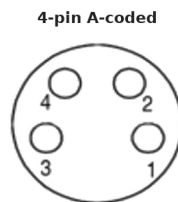
Female face view (mating side)
