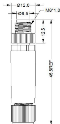
MALE, STRAIGHT
