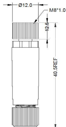
FEMALE, STRAIGHT
